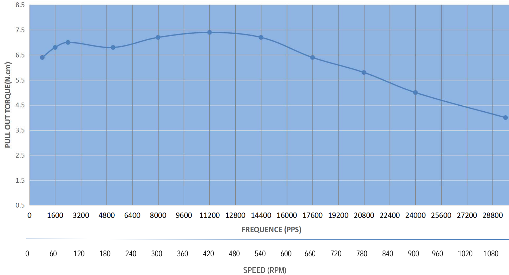
PULL OUT TORQUE CURVE OF 16HS08-0604S
