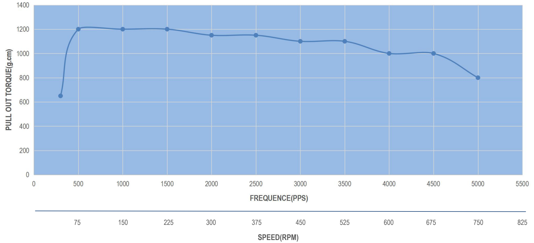
17HS08-1004S PULL OUT TORQUE(1.0A/P 24V HALF STEP)
