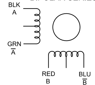
BIPOLAR SERIES
