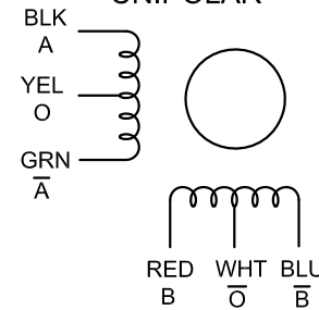
UNIPOLAR
