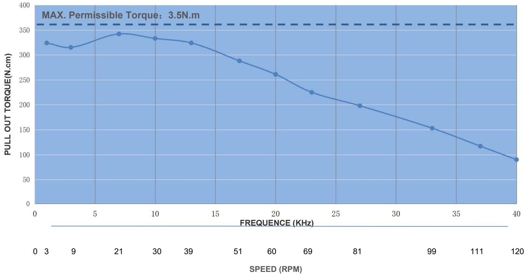
PULL OUT TORQUE CURVE OF 17HS15-1684S-HG10
