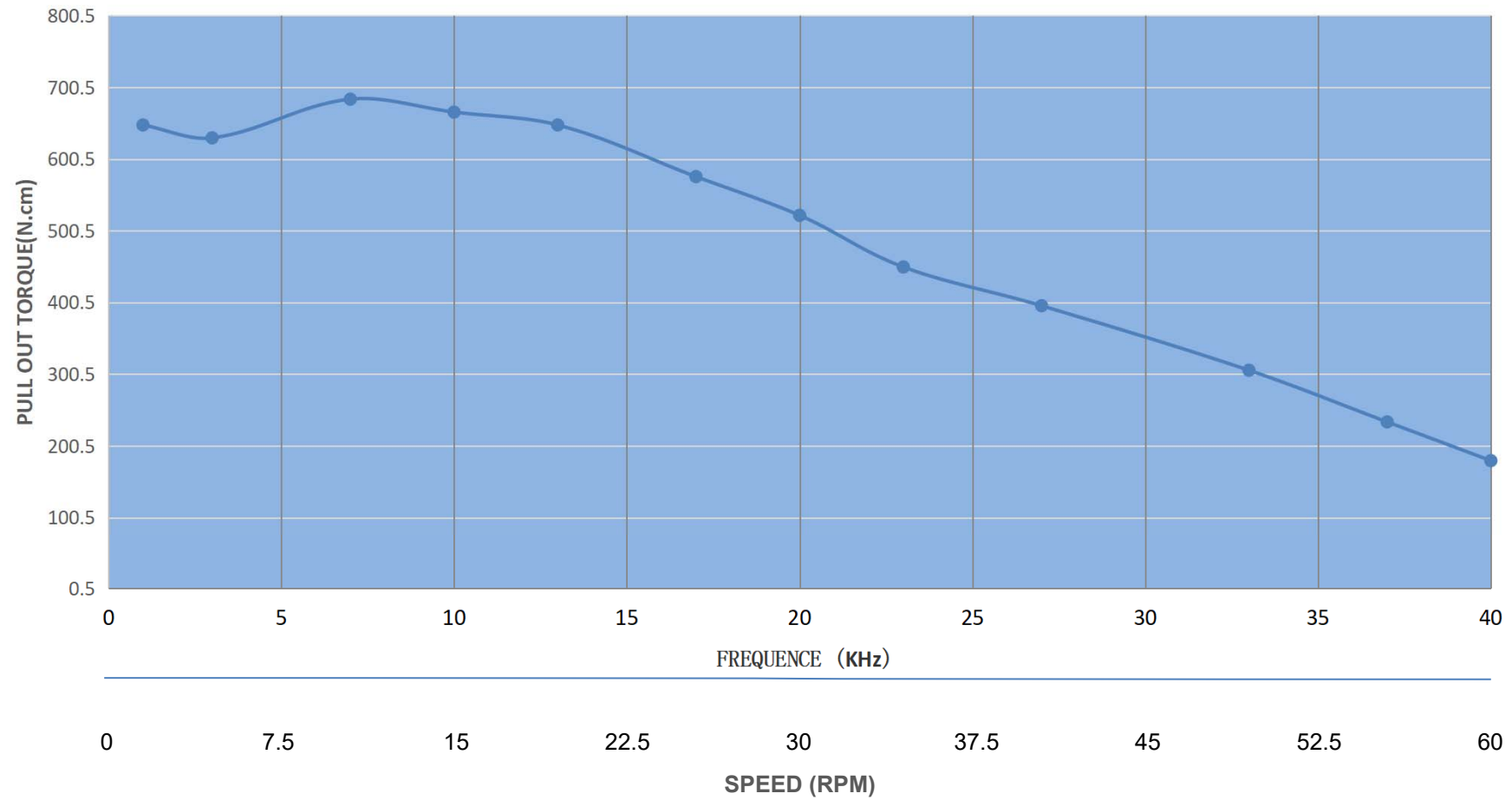
PULL OUT TORQUE CURVE OF 17HS15-1684S-HG20
