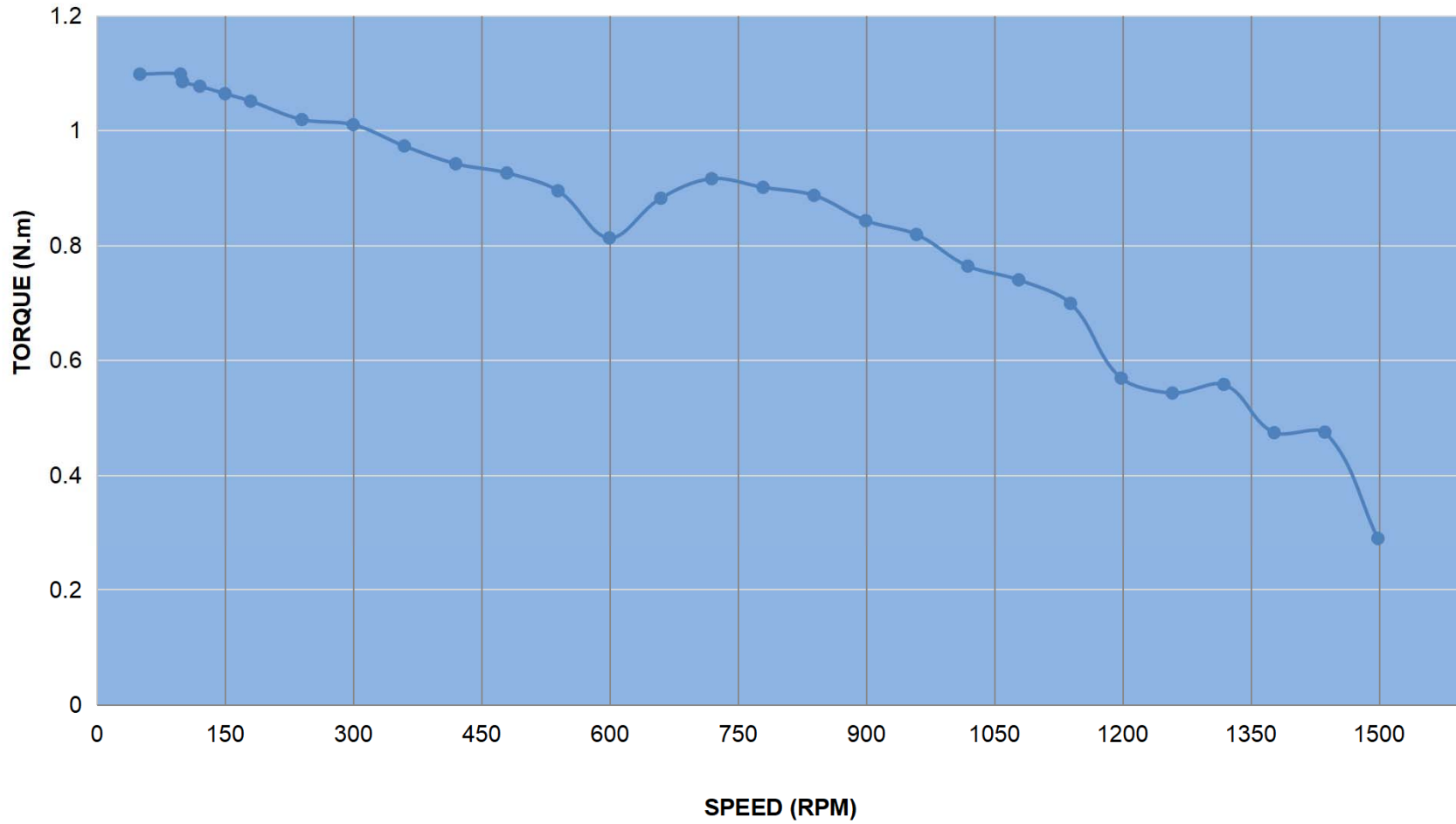
PULL OUT TORQUE CURVE OF 23E1K-12
