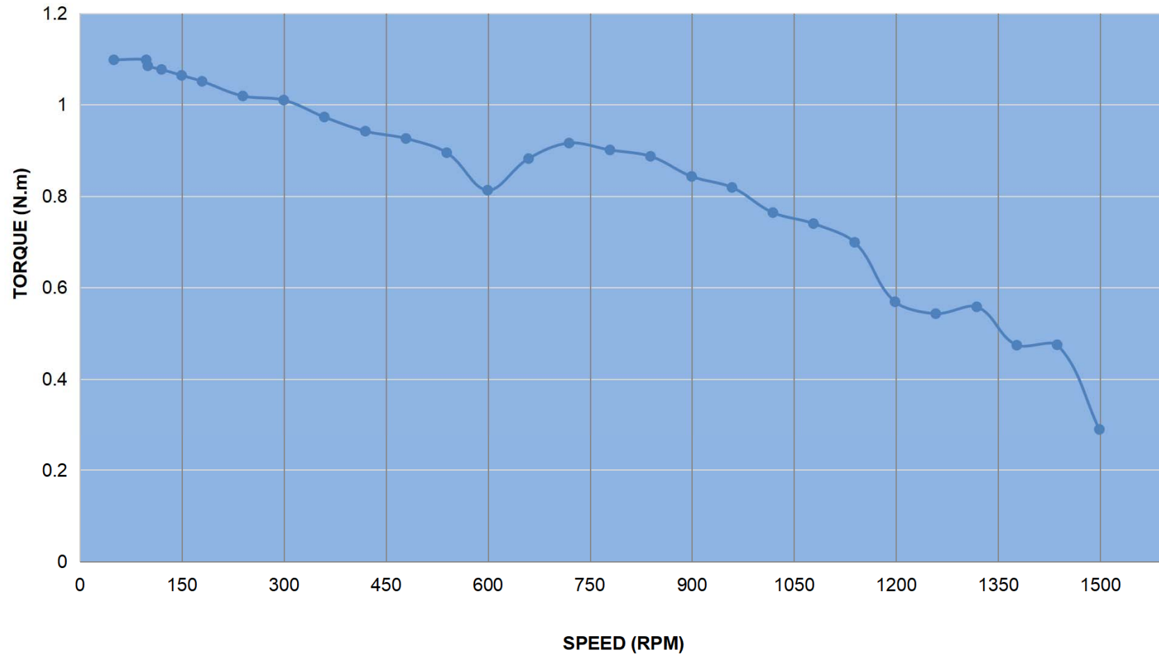
PULL OUT TORQUE CURVE OF 23E1KIP65-12
