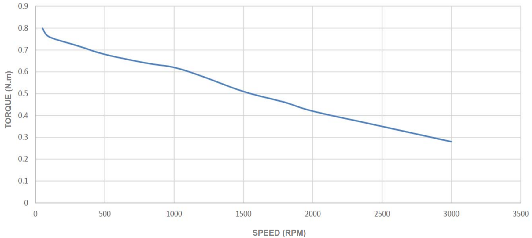
PULL OUT TORQUE CURVE OF 23HT22-5503S
