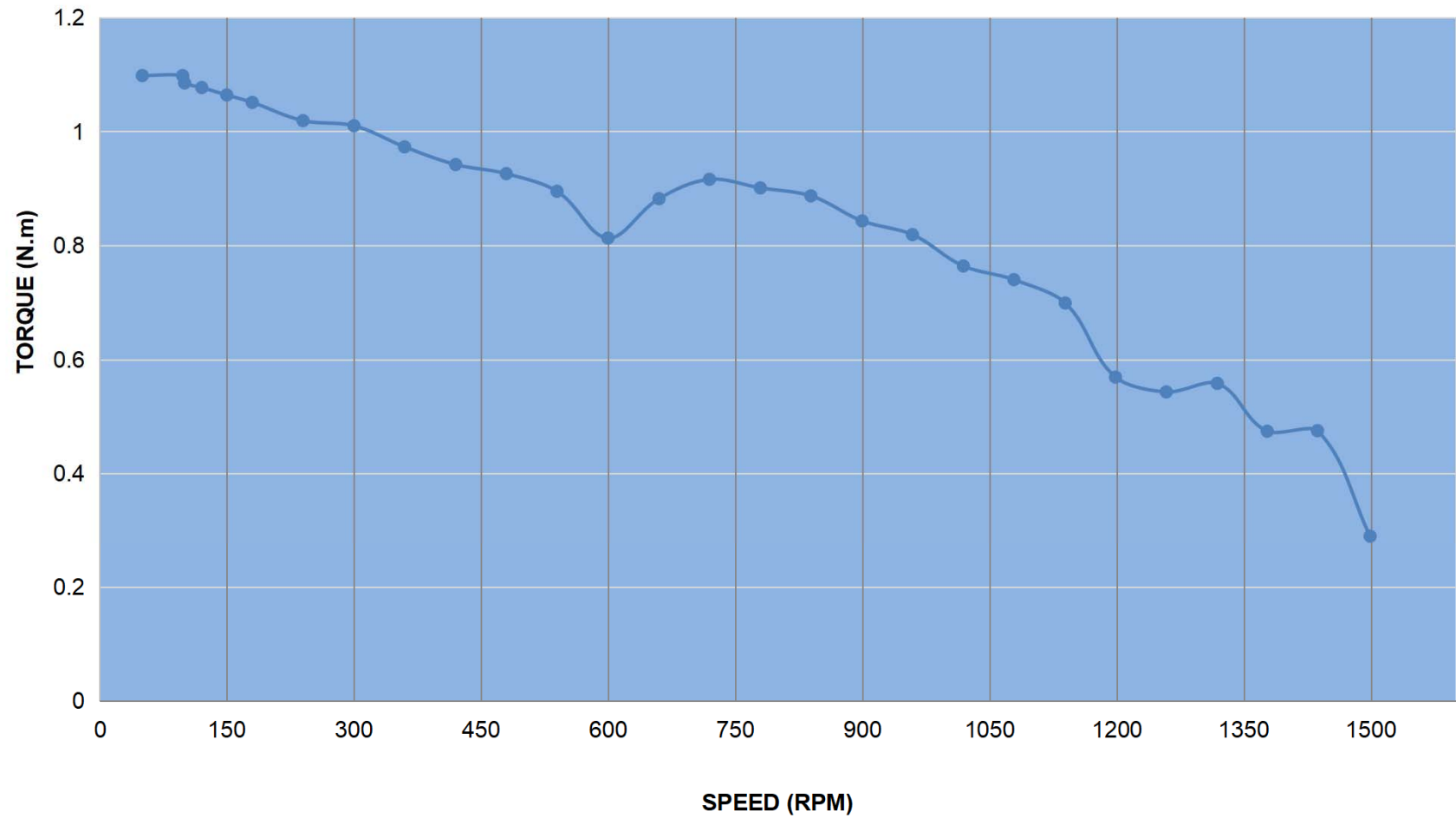
PULL OUT TORQUE CURVE OF 23IP65-12
