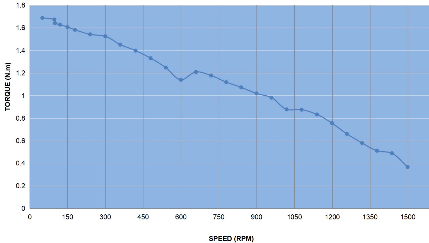
PULL OUT TORQUE CURVE OF 23IP65-20
