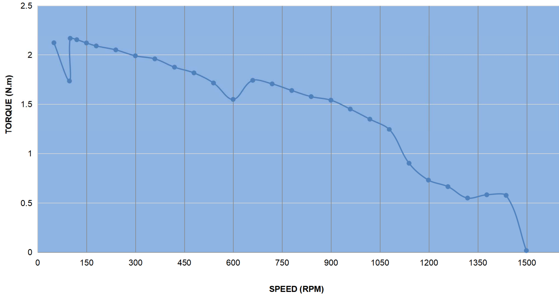
PULL OUT TORQUE CURVE OF 24BK20-30
