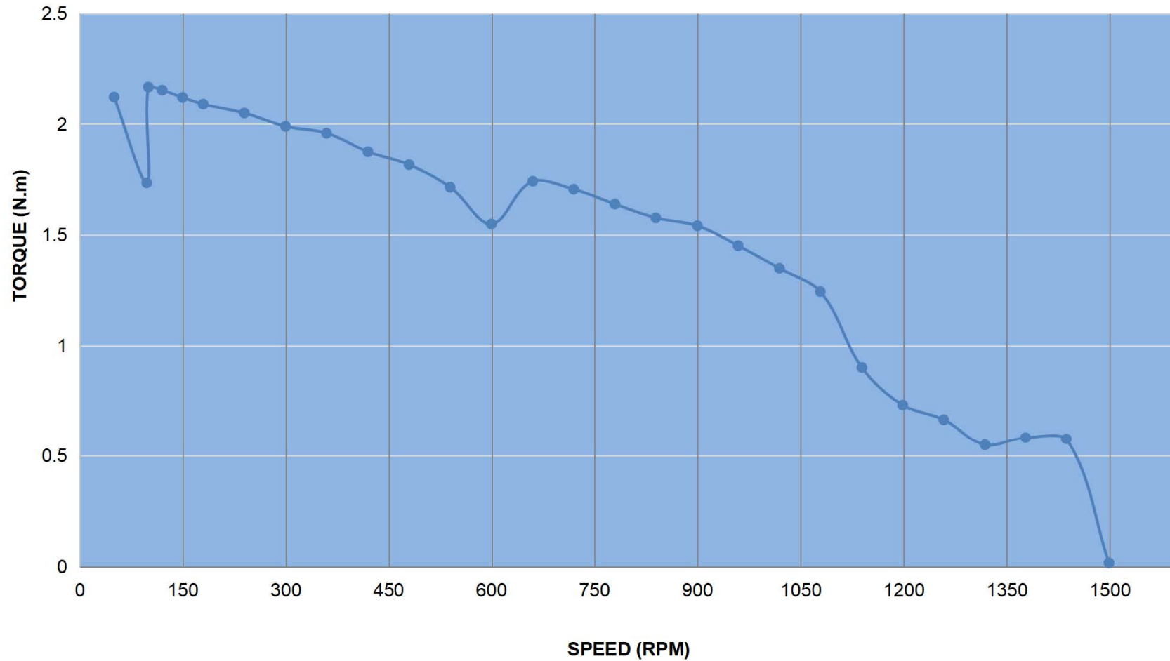
PULL OUT TORQUE CURVE OF 24E1KBK20-30
