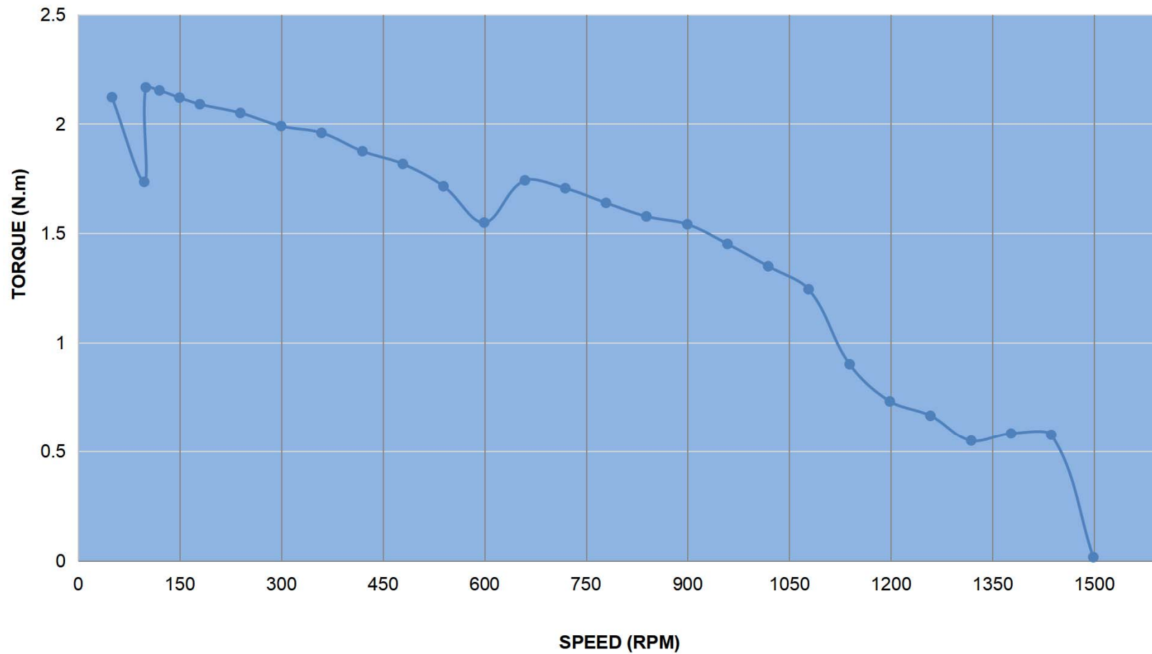
PULL OUT TORQUE CURVE OF 24E1KIP65-30
