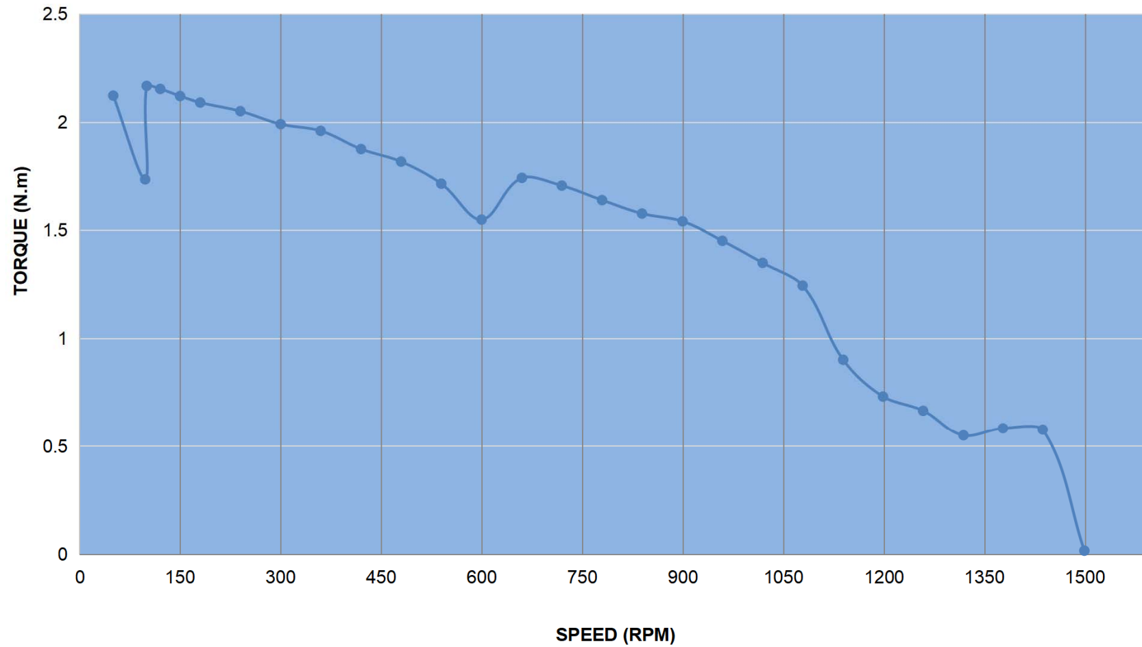
PULL OUT TORQUE CURVE OF 24IP65-30
