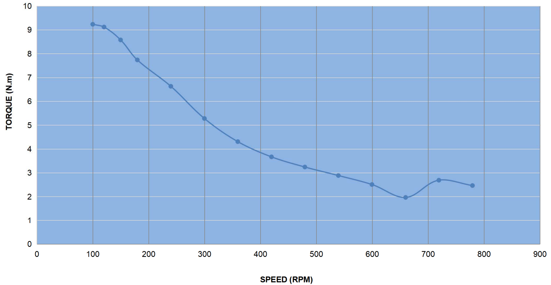
PULL OUT TORQUE CURVE OF 34BK50-120
