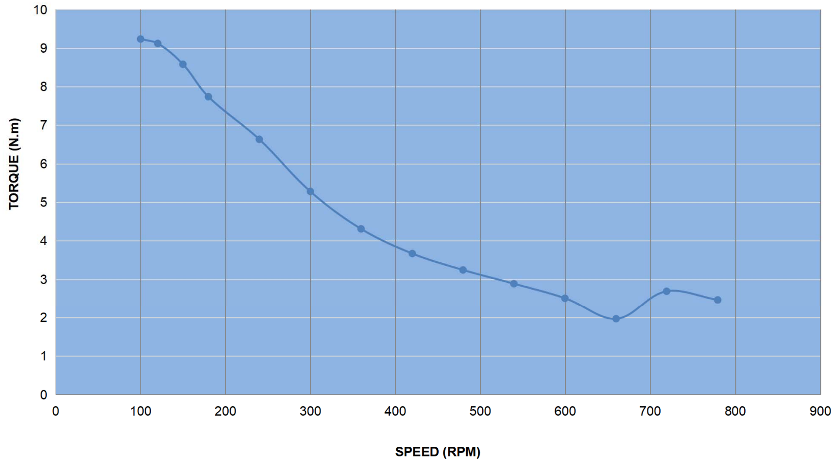
PULL OUT TORQUE CURVE OF 34E1K-120
