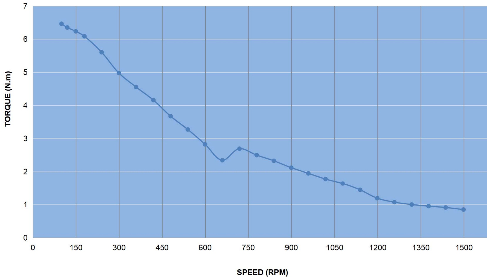
PULL OUT TORQUE CURVE OF 34E1K-85
