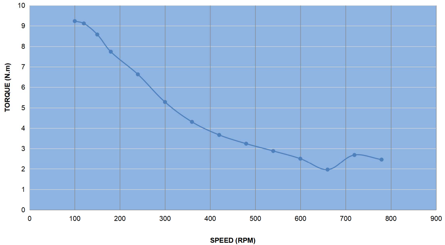
PULL OUT TORQUE CURVE OF 34E1KBK50-120
