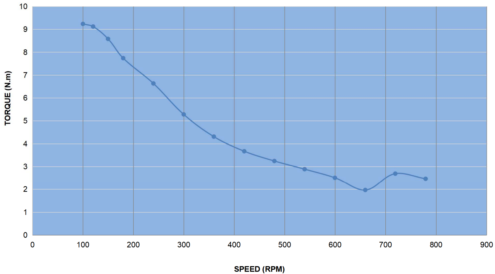
PULL OUT TORQUE CURVE OF 34E1KIP65-120
