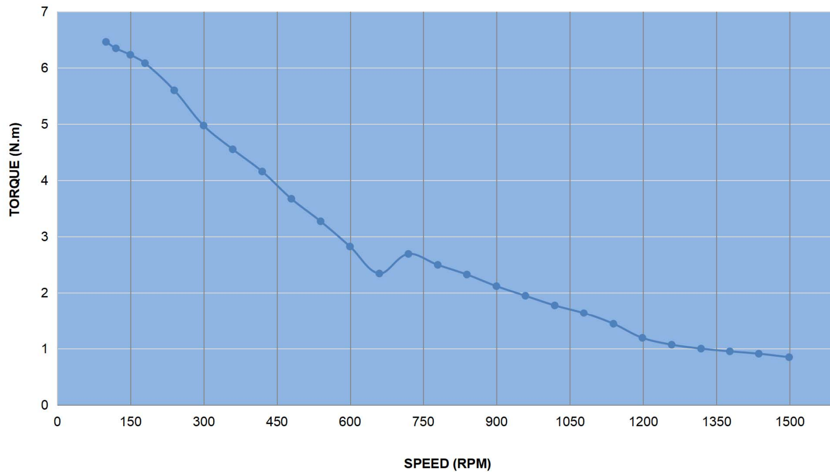
PULL OUT TORQUE CURVE OF 34E1KIP65-85
