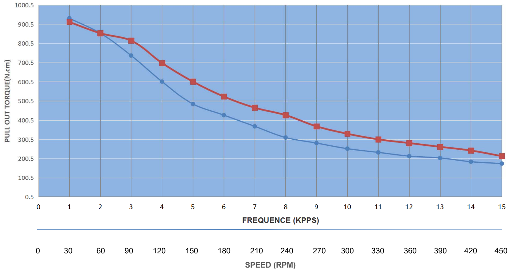
PULL OUT TORQUE CURVE OF 34HS59-5004D
