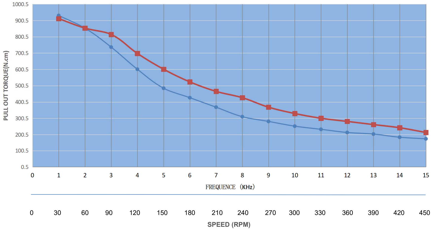
PULL OUT TORQUE CURVE OF 34HS59-5004S
