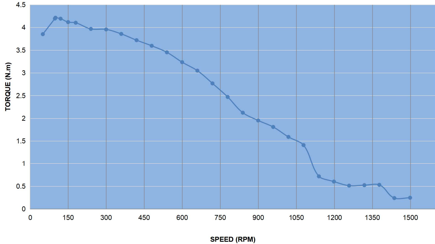
PULL OUT TORQUE CURVE OF 34IP65-45
