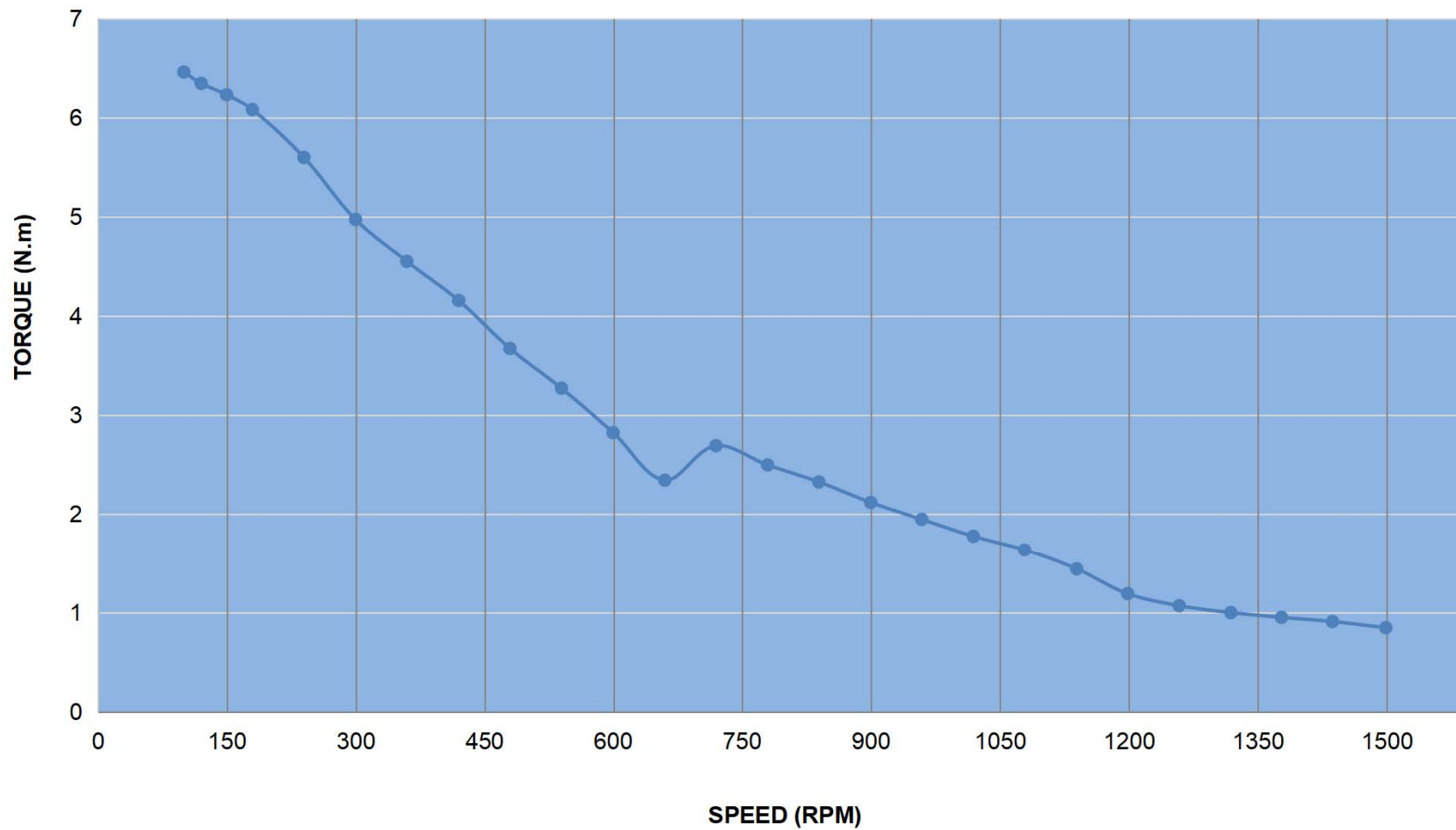
PULL OUT TORQUE CURVE OF 34IP50-85
