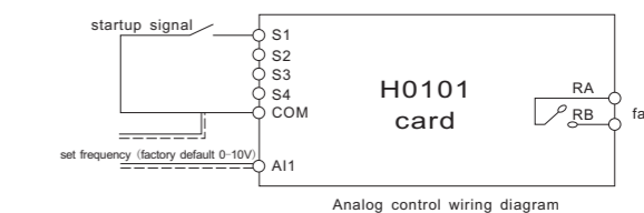
Analog control wiring diagram
