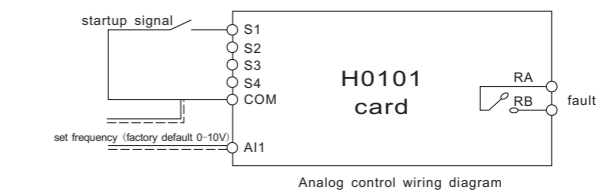
Analog control wiring diagram
